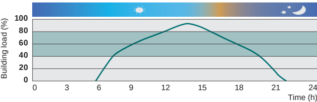
Load curve (a typical office building)
